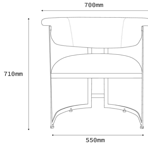
Front Elevation
